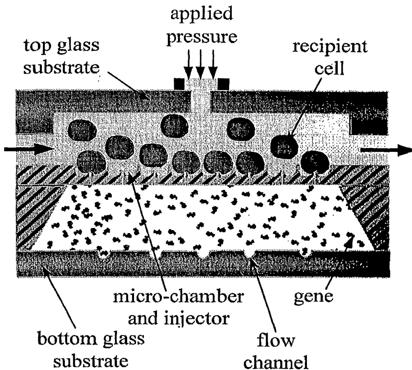
Cell Transformation Microdevice
